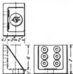
Figs. 4193-4195. Tank Stop Block Bracket.
